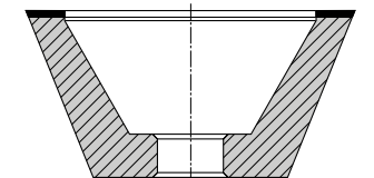
11-D-W/X FEPA 11B2
