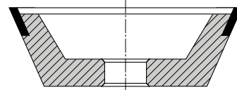
11-D-X/U-45° FEPA 12V9
