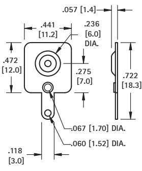
(+) POSITIVE BUTTON WITH TAB/LANCE
