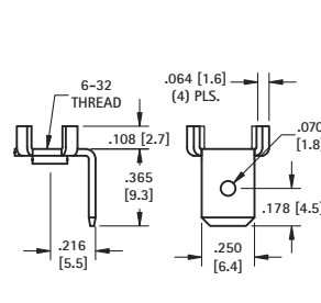
Mounting Detail
