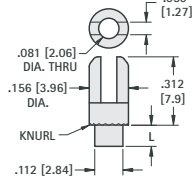
Staking Tool No. TL-9
