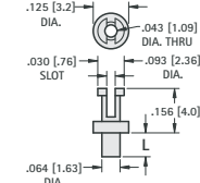
Staking Tool No. TL-2
