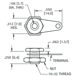
Accepts .120 (3.0) Plug
