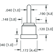
Bottom Mount
