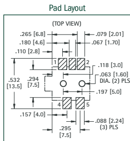
FOR 2.5 mm PLUGS
