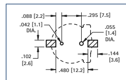
Pad Layout
