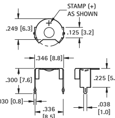
Thru Hole Mount
