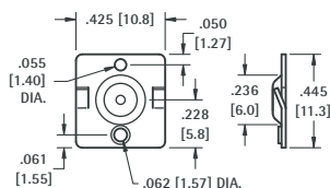
DUAL BUTTON CONTACT
