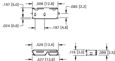
SURFACE MOUNT SOCKET
