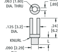
Staking Tool No. TL-3
