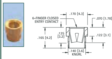
.084 (2.13) - .102 (2.6) PIN - PRESS-FIT
