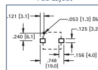
Pad Layout
