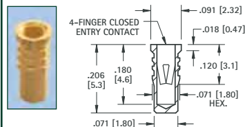
.032 (.56) - .046 (1.17) PIN - PRESS-FIT
