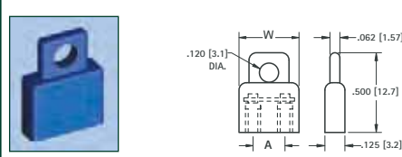
INSULATED SHORTING JACK
