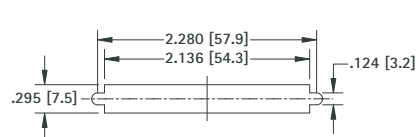
SCSI 2, 3 OR 4 - 68 PIN
