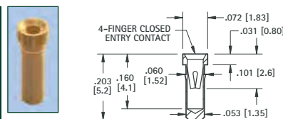
IC SOCKET CONTACTS FOR .015 (.38) - .025 (.64) LEADS - PRESS-FIT
