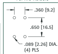
Mounting Detail For Two Holders
