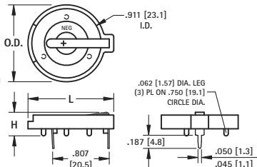
Mounting Detail
