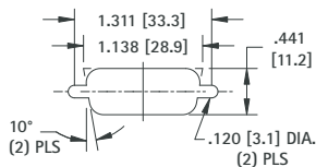
SCSI 1 - 50 PIN
