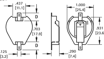
Surface Mount
