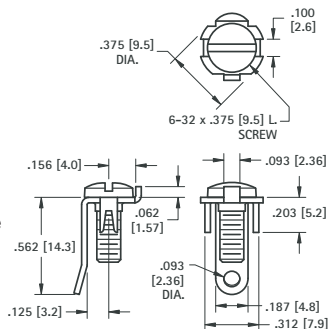
SOLDER TAB
