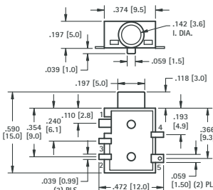
FOR 3.5 mm PLUGS
