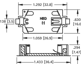
Surface Mount
