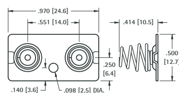
DUAL SPRING CONTACT
