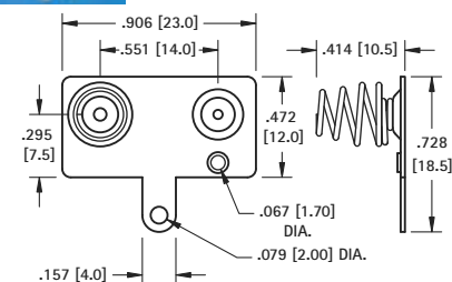
DUAL CONTACT WITH TAB/LANCE
