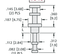
Staking Tool No. TL-12
