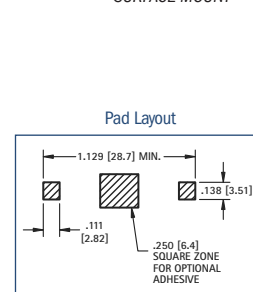
Pad Layout
