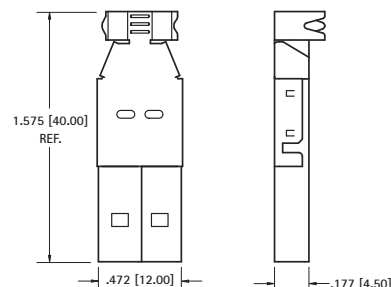
CABLE PLUG
