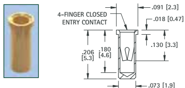
.032 (.81) - .046 (1.17) PIN - SOLDER MOUNT
