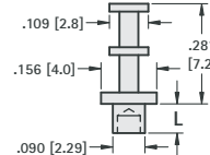
Staking Tool No. TL-5
