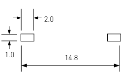
Recommended pad size
