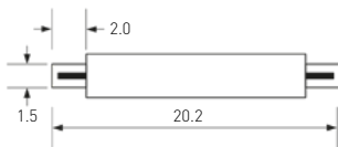
Recommended pad size
