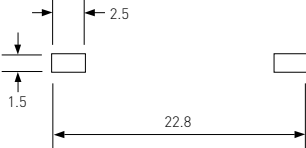
Recommended pad size
